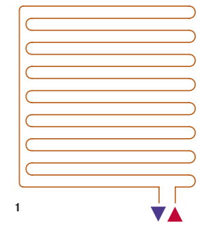
1 _ Zig-zag: suitable for rooms with irregular floor surfaces. The inter-tube spacing can be easily reduced for areas where more concentrated heat is required.
