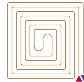
3 _ Spiral: ensures that heat is distributed in a uniform manner. It is recommended for regular surfaces.
